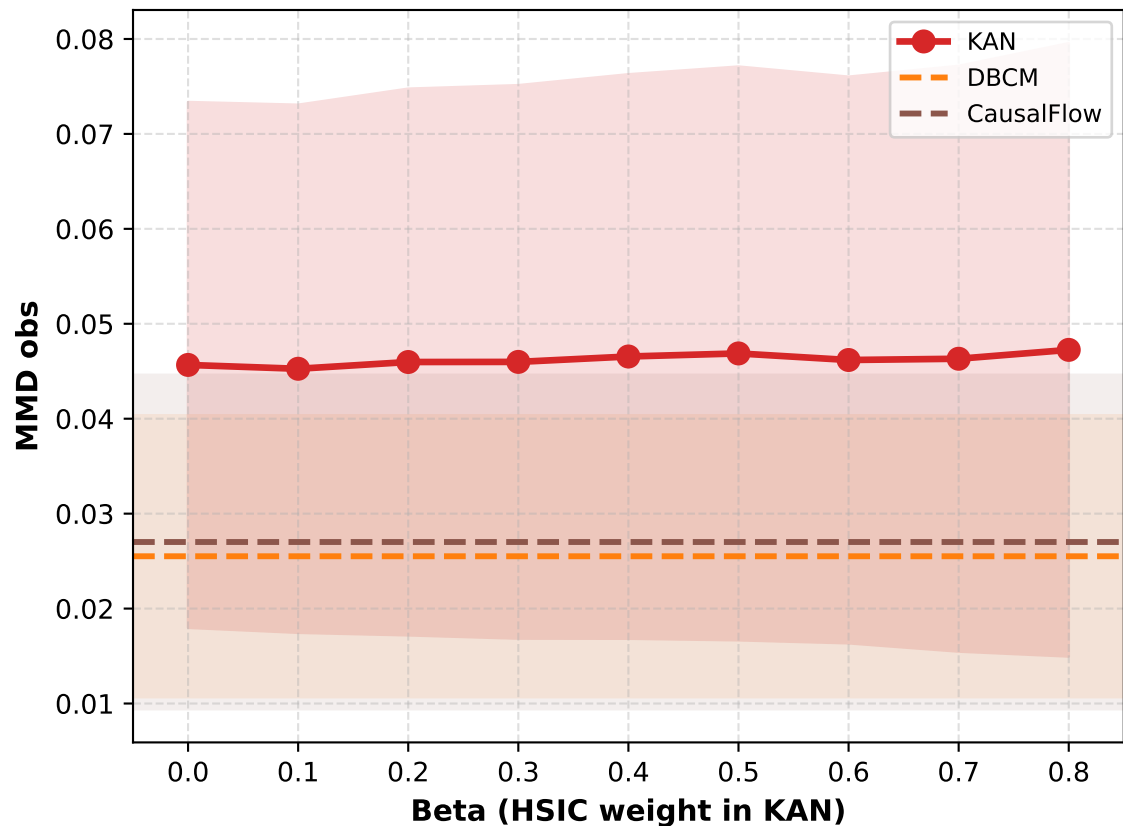
MMD obs
